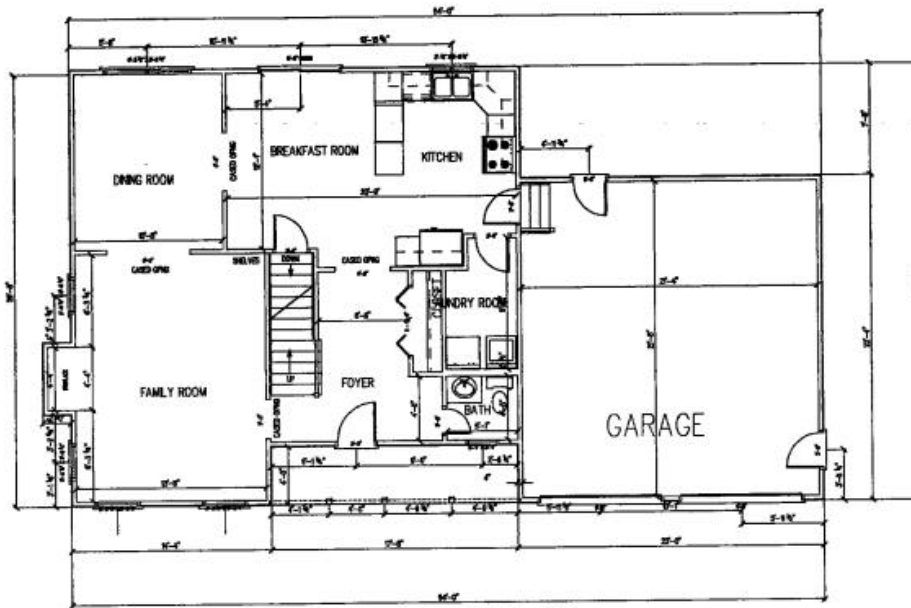
1ST FLOOR FLOOR PLAN
